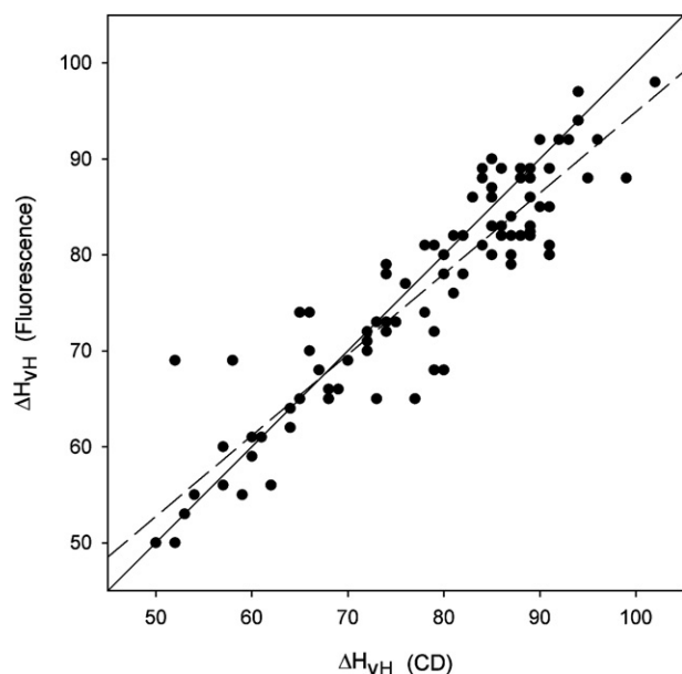
Fig. 3. Plot of van't Hoff enthalpies in units of kcal/mol calculated from fluorescence thermal denaturations versus those calculated from circular dichroism thermal denaturations. The solid line is that upon which all points would fall if there were perfect correspondence in the two values. The dashed line is the result of a least square fit. The slope of this regression line is 0.8441, the Y-intercept is 10.436, and the value of r^2 is 0.8441.
