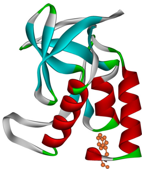
Fig. 1. Ribbon diagram of staphylococcal nuclease (PDB 1EY0) with tryptophan 140 shown in orange. Helical secondary structure is shown in red. (For interpretation of the references to colour in this figure legend, the reader is referred to the web version of this article.)
