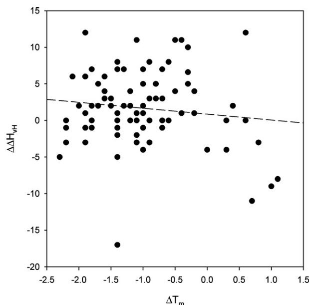
Fig. 4. Plot of the difference in midpoint temperatures from fluorescence and circular dichroism thermal denaturations (in units of °C) versus the difference in van't Hoff enthalpies for the same denaturations (in units of kcal/mol). The dashed line is the result of a least square fit. The slope of this regression line is -0.88 , the Y-intercept is 0.73, and the value of r^2 is 0.019.
