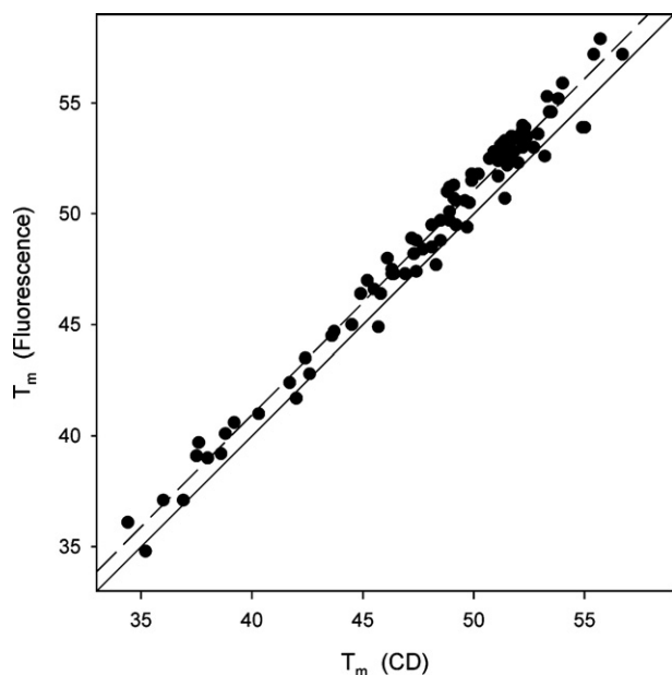
Fig. 2. Plot of midpoint temperature in units of °C calculated from fluorescence thermal denaturations as a function of midpoint temperature calculated from circular dichroism thermal denaturations. The solid line is that upon which all points would fall if there were perfect correspondence in the two values. The dashed line is the result of a least square fit. The slope of this regression line is 1.012, the Y-intercept is 0.463, and the value of r^2 is 0.9787.
